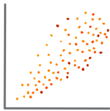
SCATTERPLOT
