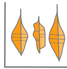
VIOLINPLOT
