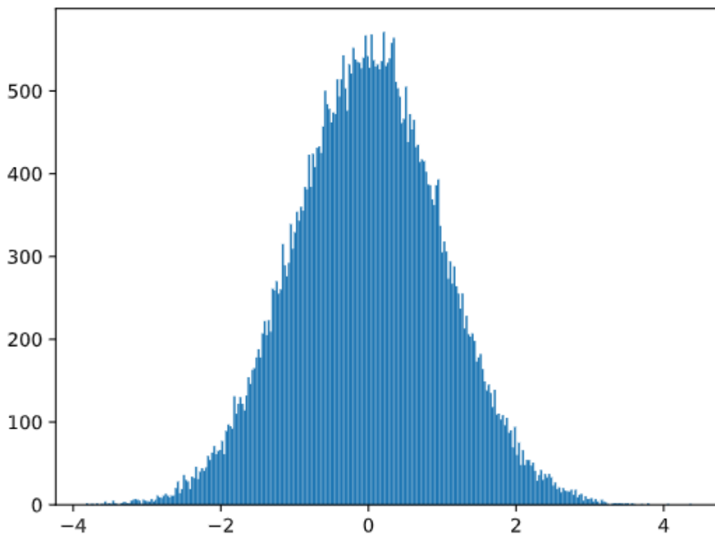
Normal Distribution with mean=0 and std.dev=1
